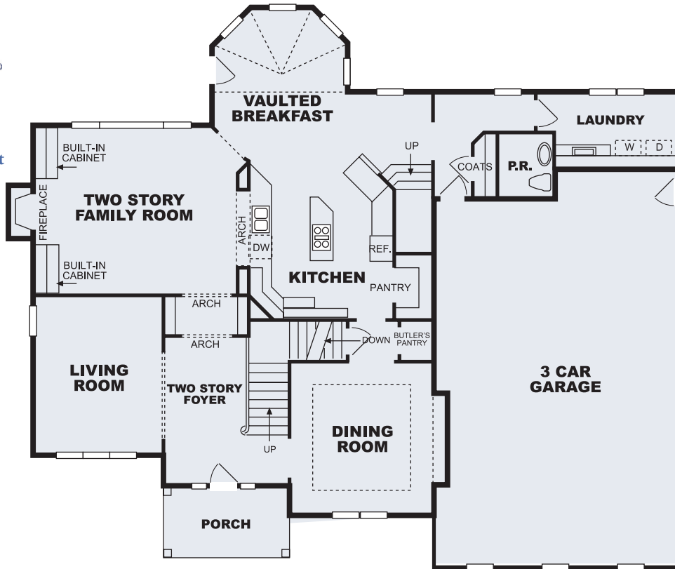
FIRST LEVEL
